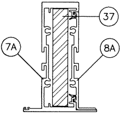
MULLION 'M5' (LEVEL 'D' IMPACT)
