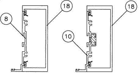
STD. DOOR MULLION W/O REINF. (LEVEL 'D' IMPACT)
