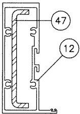
JAMB 'J2' (LEVEL 'D' & 'E' IMPACT)
