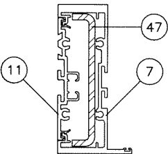
JAMB 'J2A' (LEVEL 'D' & 'E' IMPACT)
