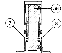
MULLION 'M2' (LEVEL 'D' & 'E' IMPACT)
